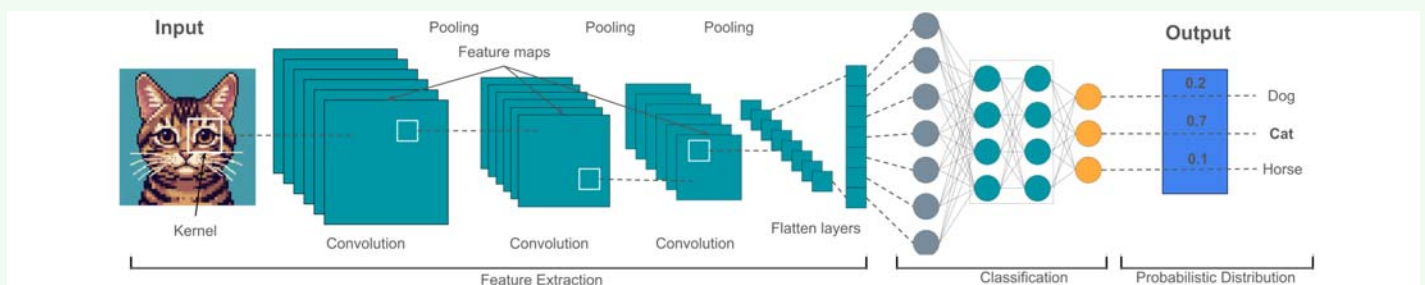
The CNN Architecture
